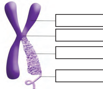
2.5 Chromosome
