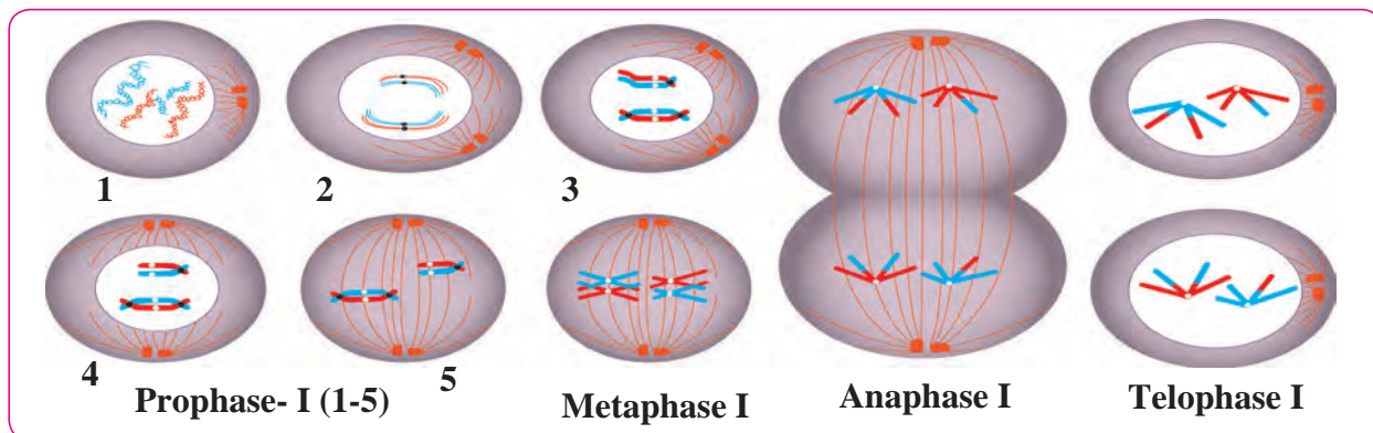
2.8 Meiosis Part-I
